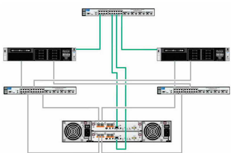
Figure 22. MSA 2040/2042 SAN iSCSI Network
