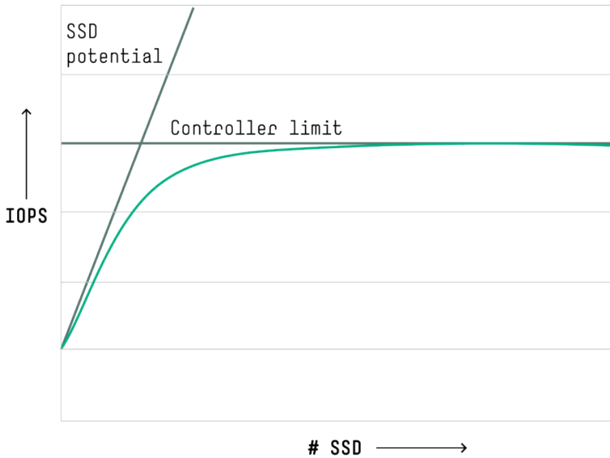
Figure 21. SSD performance potential vs. MSA 1040/2040 controller limit
