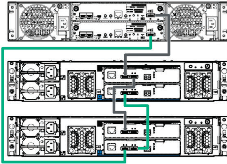
Figure 20. Reverse cabling example using the HPE MSA 1040 system
