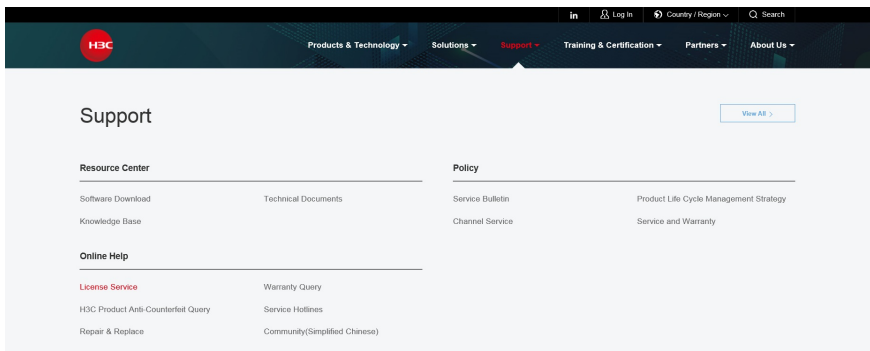
Figure 13 Product licensing
